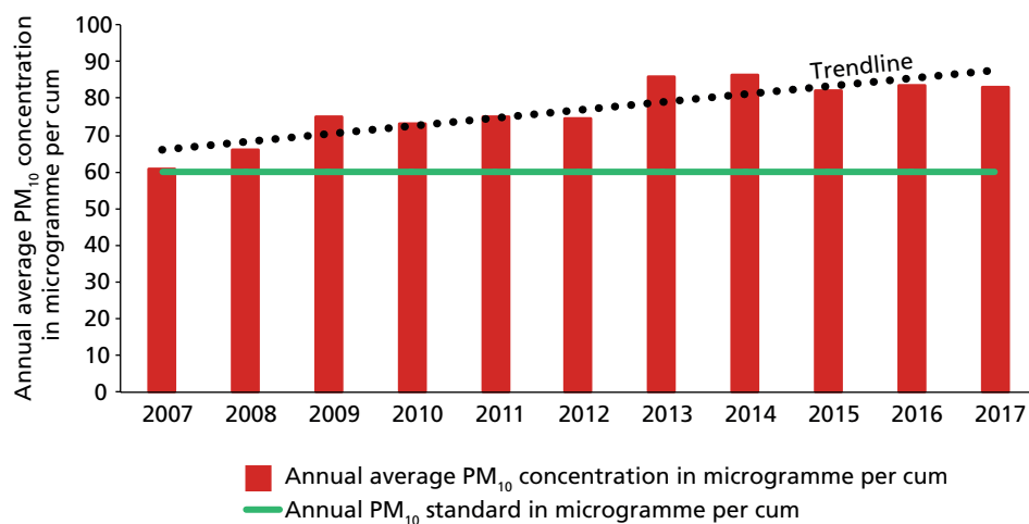
Graph 3B: Balasore—long-term trend in annual average level of PM 10 concentration
