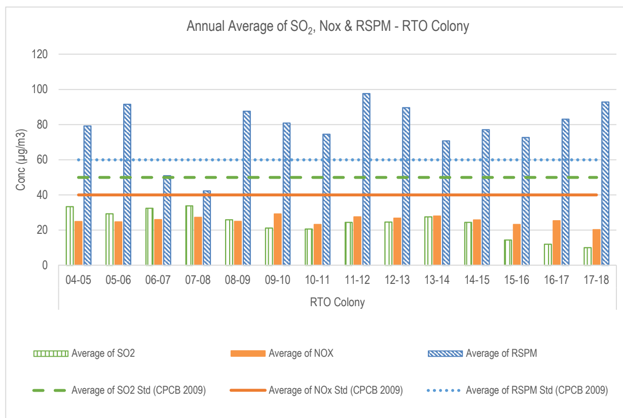
Figure: Annual average trend of SO 2 , NO x , and RSPM at RTO Colony
