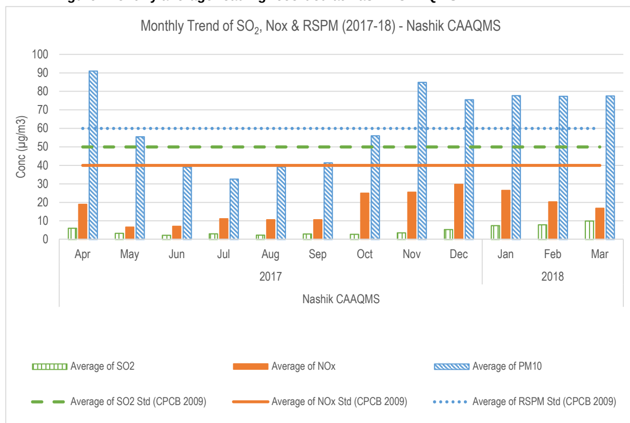
Figure: Monthly average reading recorded at Nashik CAAQMS
