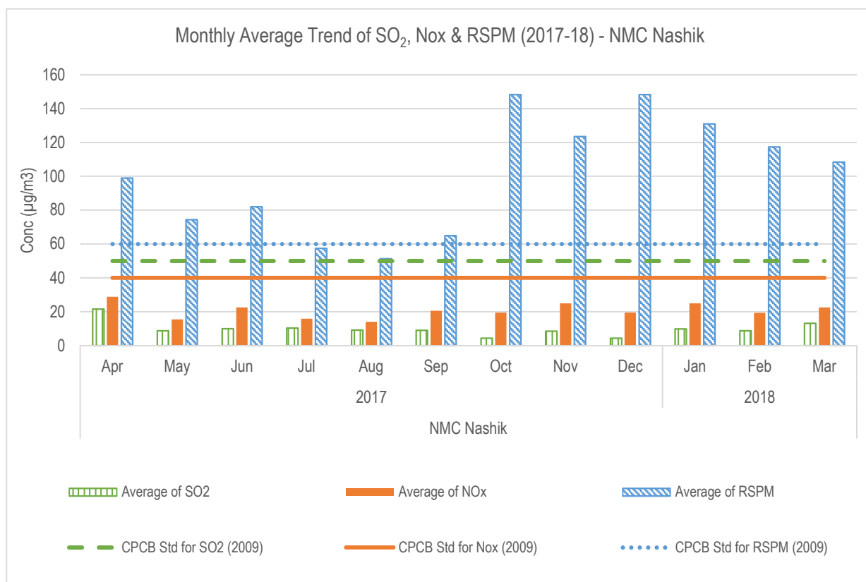
Figure: Monthly average reading recorded at NMC Nashik
