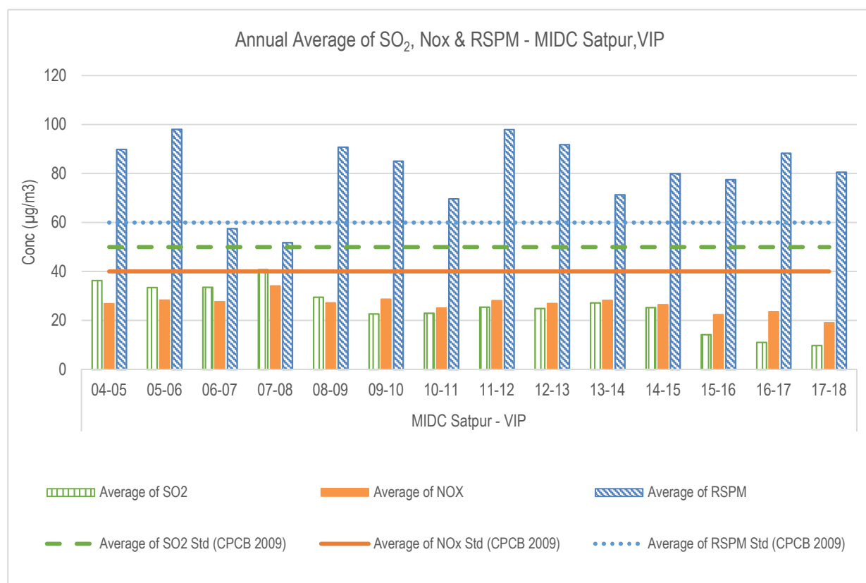
Figure: Annual average trend of SO 2 , NO x , and RSPM at MIDC Satpur - VIP
