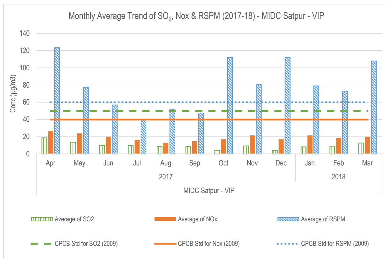
Figure: Monthly average reading recorded at MIDC Satpur - VIP
