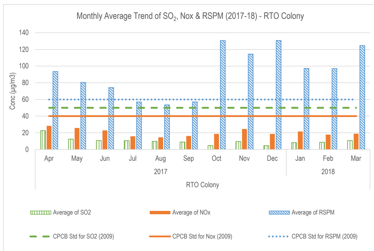
Figure: Monthly average reading recorded at RTO Colony
