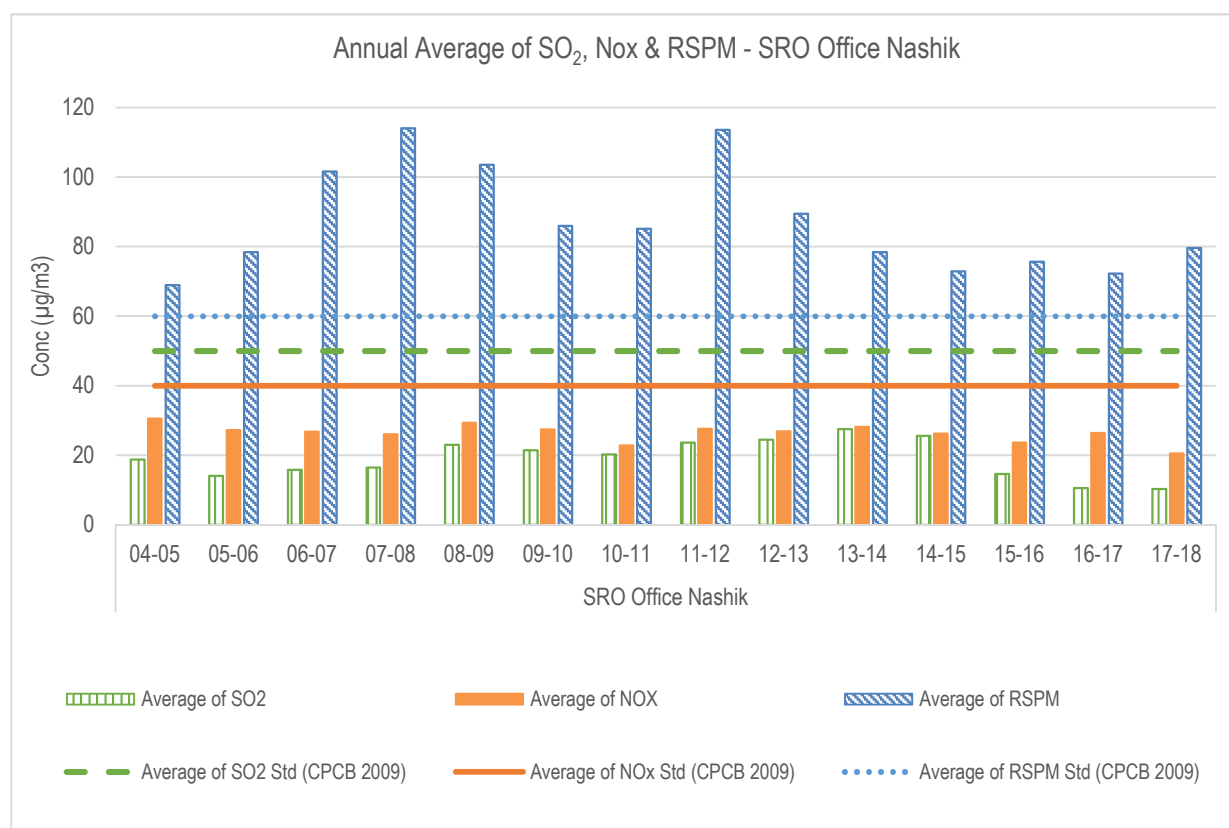
Figure: Annual average trend of SO 2 , NO x , and RSPM at SRO Office Nashik
