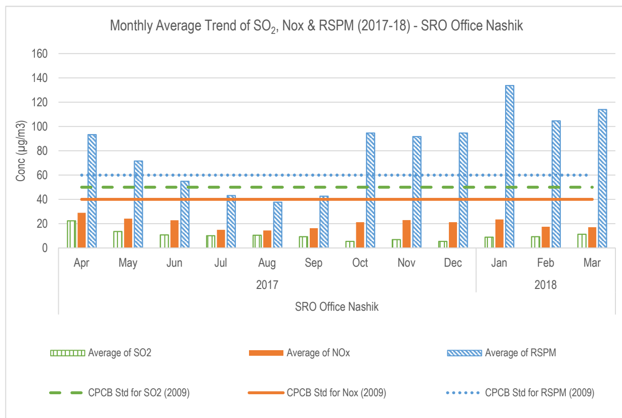
Figure: Monthly average reading recorded at SRO Office Nashik
