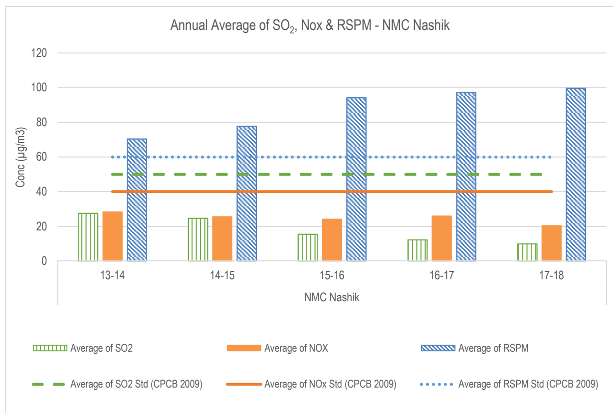
Figure: Annual average trend of SO 2 , NO x , and RSPM at NMC Nashik
